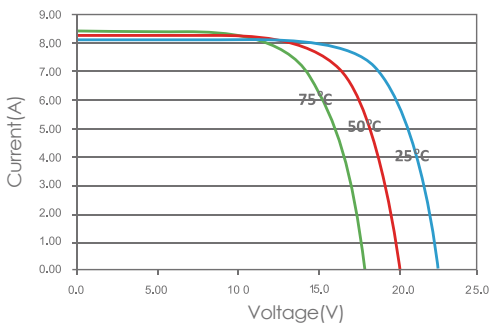
I-V Curves of PV Module GES-6P140 at Different Cell Temperatures(AM1.5,1000W/m 2 )
